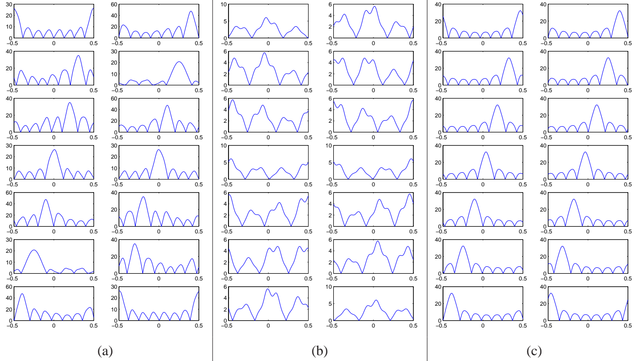
Fig. 9. Third example (in the MCLT case with window h_{a_2} ): frequency responses of synthesis filters (a) before and after optimization (b) with the cost function \widetilde{J}_{ts} and (c) with J_{ts} .
