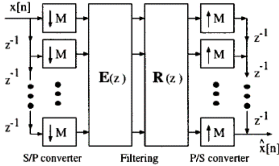
Fig. 3. Block diagram of the M -channel maximally decimated filter bank from Fig. 2 with polyphase implementation.
